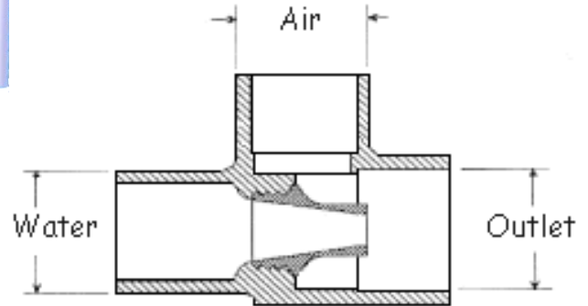
Front View of VT4090-1
