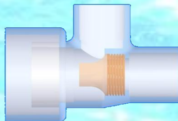
Part # VT40 (1 1/2 "-1") soc x 1" spt x 1" spt 3/4" soc
