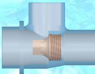
Part # VT40-1 Venturi Tee PVC 1" soc x 1" spt x 1"spt / 3/4" soc
